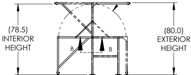
Vertical lift gate
